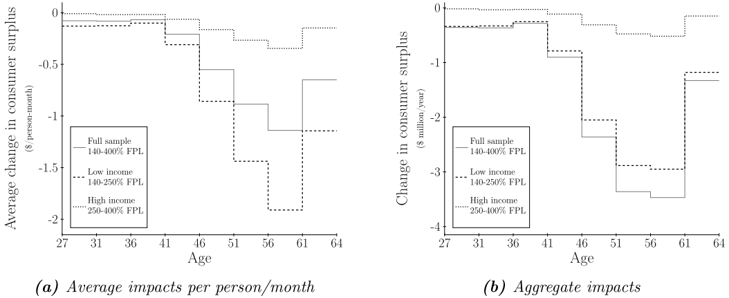
FIGURE 6.—Upper bounds on the change in consumer surplus from removing Silver plans. Notes: Each line indicates the estimated nonparametric upper bound on the change in consumer surplus for a different income group. The nonparametric lower bound is infinite.
